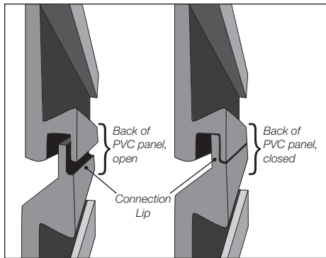
Back panel connection lip ↴
