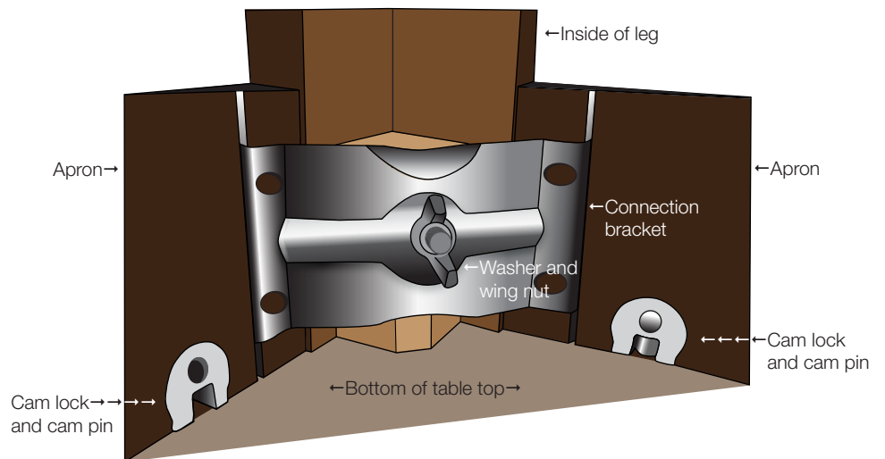
Connection bracket in place with wing nut and washer. Cam locks in position to hold aprons to table top
