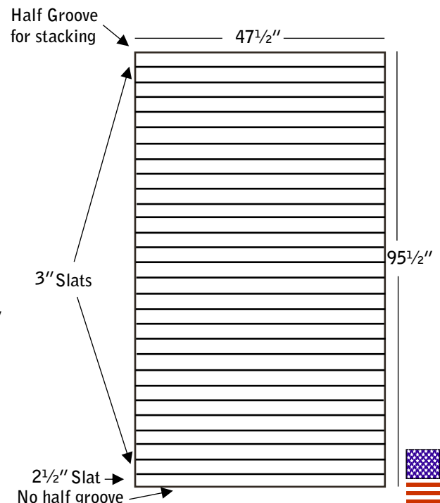
Clear coated OSB with metal groove
