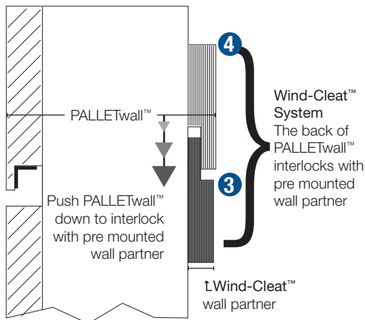
PALLETwall™ Wind-Cleat™ System
